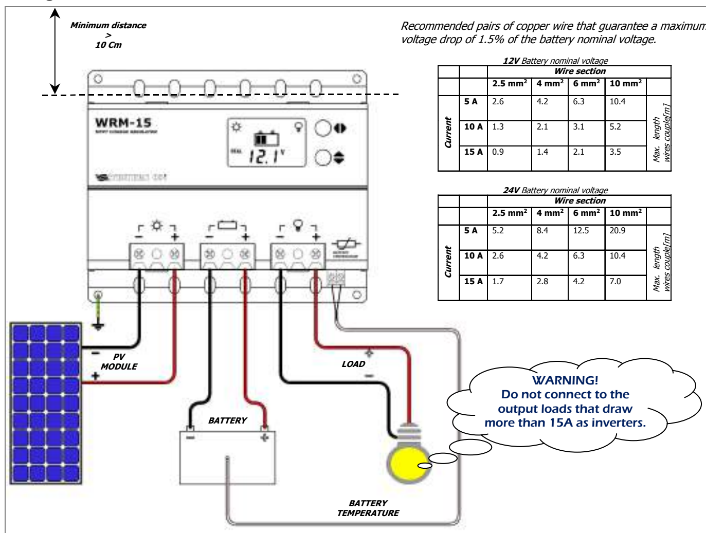
Fig. 2 Connection scheme
