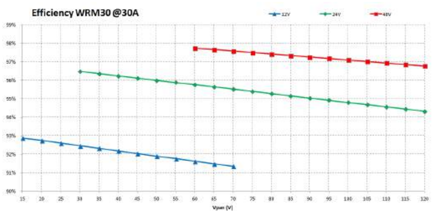
Graph. 2 Efficiencies
