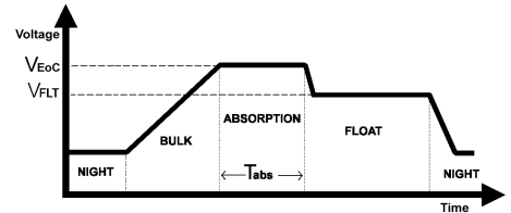
2 Graph - charging phases:
